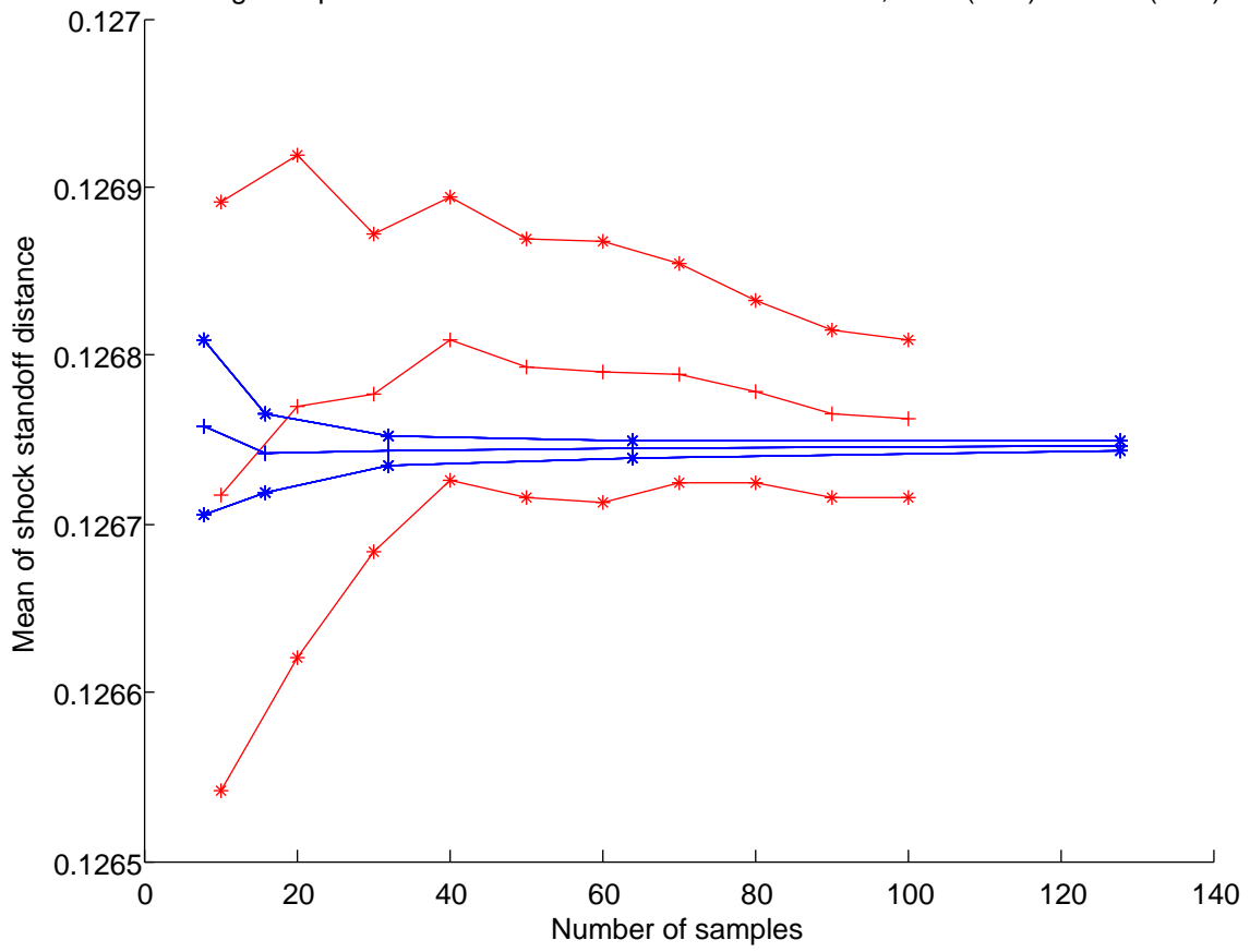
Convergence plot for the mean of shock standoff distance, SRS (Red) vs LHS (blue)
